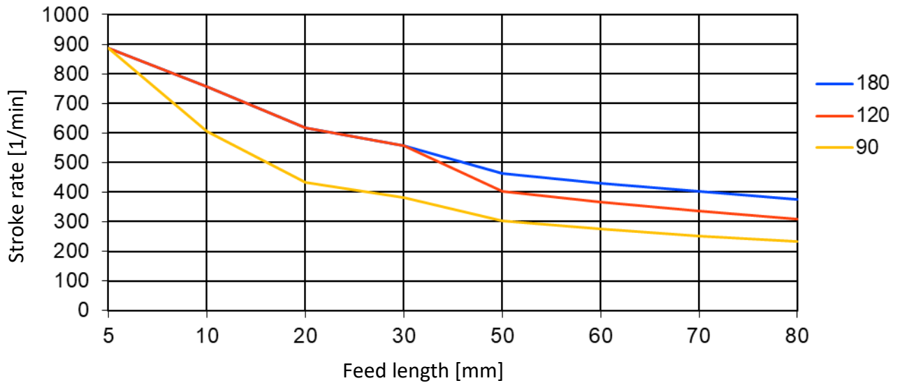
Stroke rate diagram without pilot release with belt weight 0.1kg
